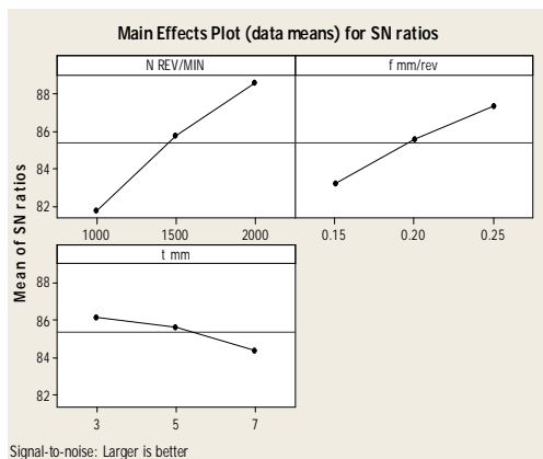
Figure No: 3.1 Effect of process parameters on S/N Ratio
