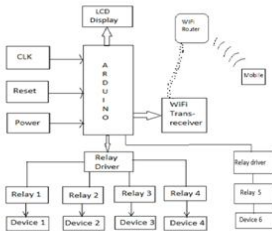
Fig 3:-Proposed Block Diagram of Industrial Automation using IOT
