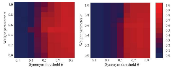
Fig. 4. Influence of threshold and weight parameters u and a . The two heat-maps represent F1 scores in different data distributions.
