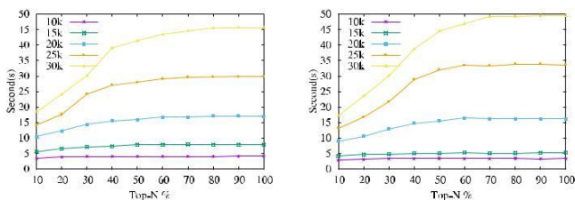
(a) The process time under different query numbers of the CA dataset (b) The process time under different query numbers of the FB dataset
