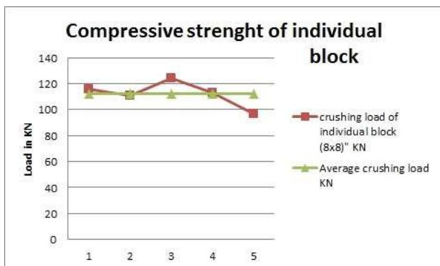
Figure 3. Graph.2 Compressive strength of individual block.
