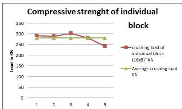
Figure 2. Graph.1 Compressive strength of individual block.
