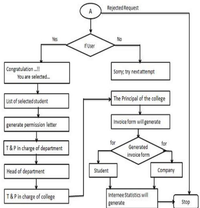
FIG 2.B. FLOWCHART OF PCE-INTERNS(Continued..)
