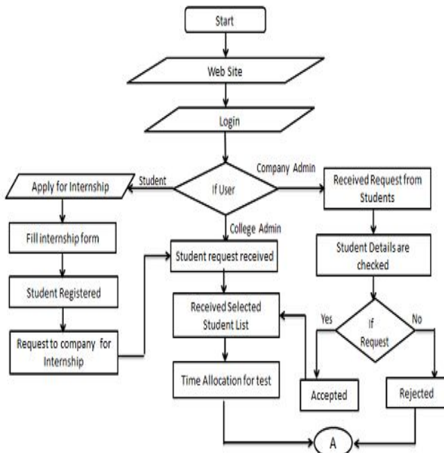
FIG 2.A. FLOWCHART OF PCE-INTERNS
