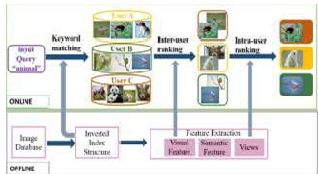
Figure 2. The system framework of tag-based image retrieval with social re-ranking.
