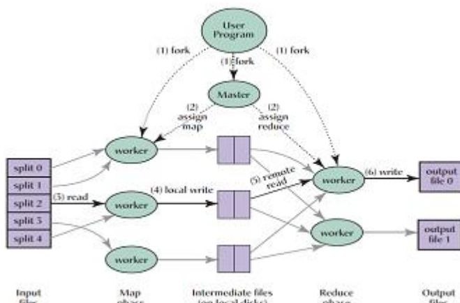
Fig:1 Map Reduce Architecture
