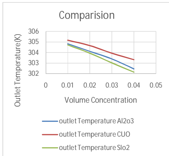
Plot 3 Graphical representation of Temperature outlet in nano fluids
