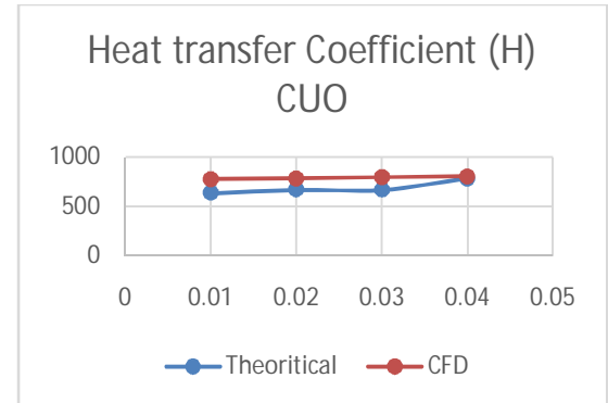
Plot 2: Comparisons of Theoretical and Computational Heat transfer coefficient of CUO
