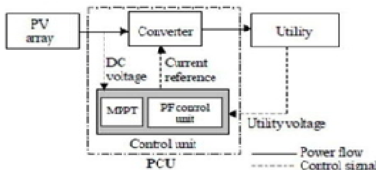
Fig.2: Schematic Diagram of Grid-Connected System
