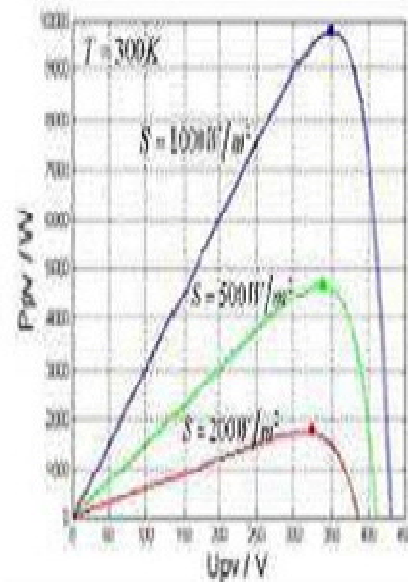
Fig.4: Photovoltaic Module P-V Characteristics
