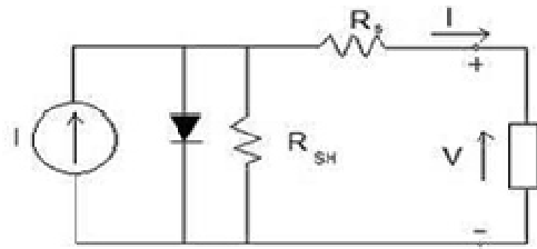
Fig.1: Equivalent Circuit Model of Cell
