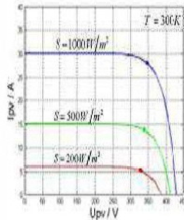
Fig.3: Photovoltaic Module I-V Characteristics
