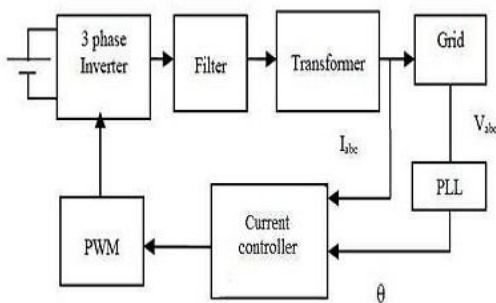
Fig 5: Block diagram of the system
