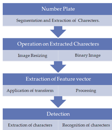
Fig.4: detection algorithm
