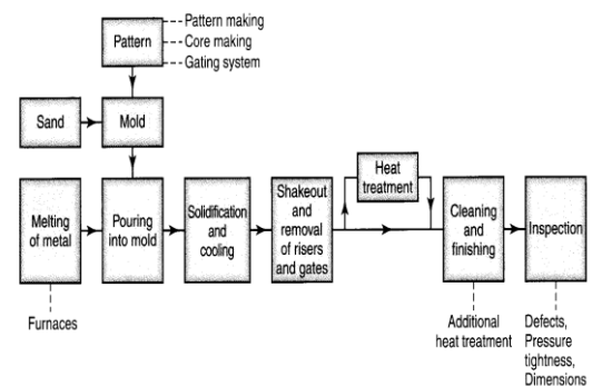
FIG.1. Outline of production steps in a typical sand-casting operation
