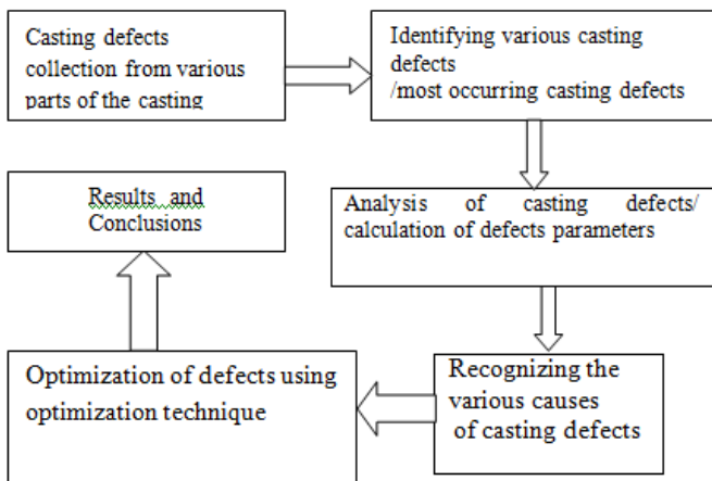
Fig. 6 METHODOLOGY
