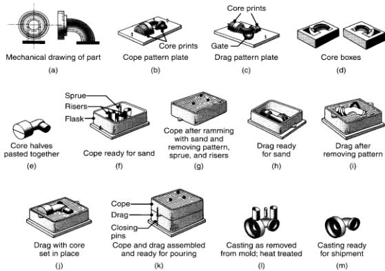
Fig.2. Schematic illustration of the sequence of operations for sand casting.
