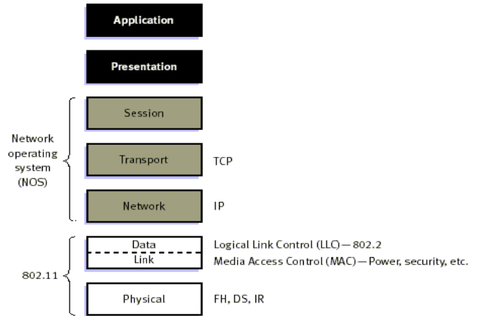
Figure 2: IEEE 802.11 and the ISO Model
