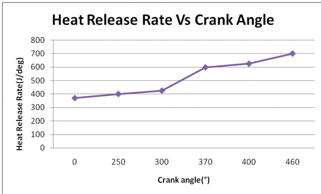
Figure 4.1: Total Heat Release rate Vs Crank Angle
