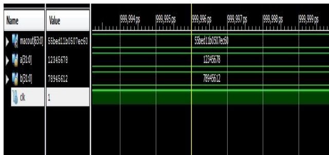
Fig 9 : Simulation result of 64 bit MAC unit
