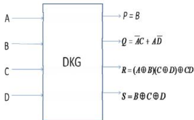
Fig 4. DKG gate
