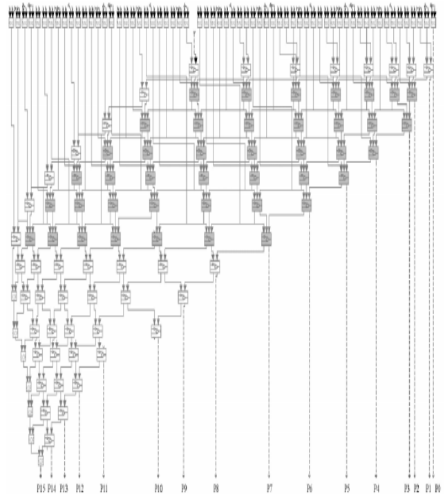
Fig 2: Hardware architecture of UrdhvaTiryakbhyam multiplier with full adders and half adders
