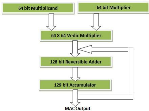
Fig 1: Modified MAC Architecture
