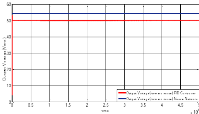
Fig 16: Comparison result of output voltage(forward mode)
