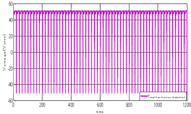
Fig 10: THD generation in buck mode
