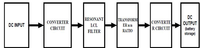
Fig 2 :- Block diagram of Forward Mode Conduction
