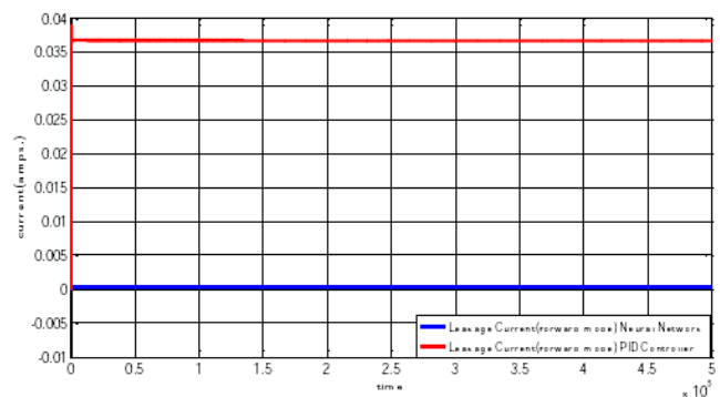
Fig 18: Leakage current comparison result
