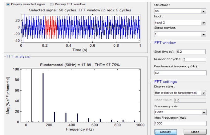
Figure 6. THD from source it is 97.75%
