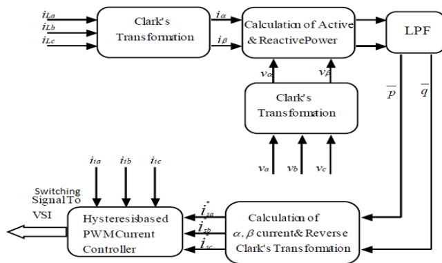
Figure 2. Instantaneous Reactive Power (IRP)
