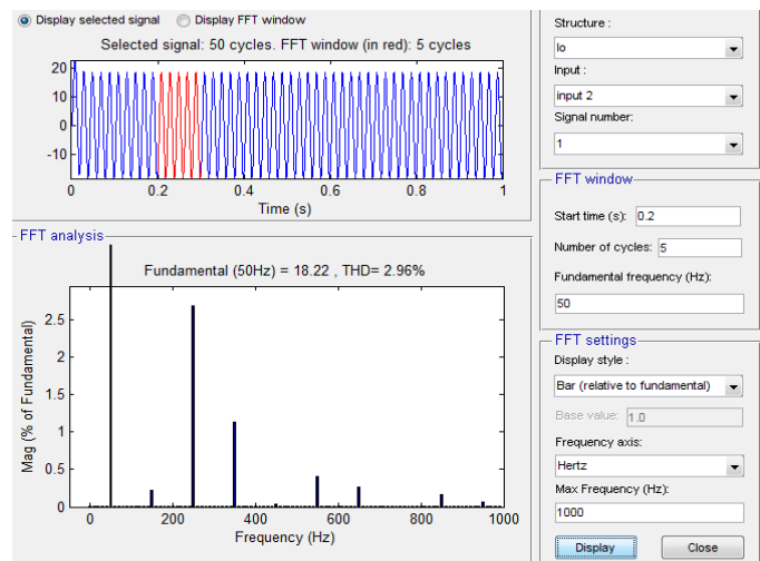
Figure 7. THD from load side it is 2.96%
