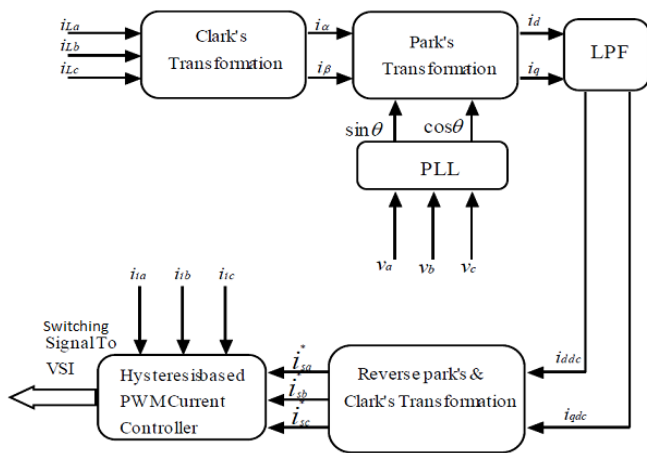
Figure 3. Synchronous Rotating Frame (SRF) Theory
