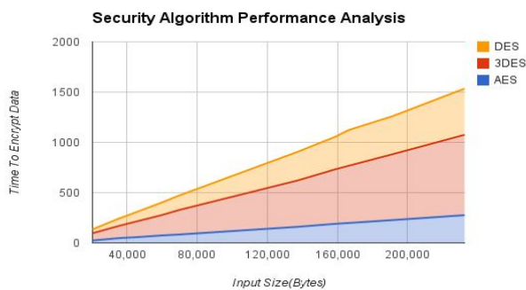
Fig. 2: Performance Analysis for security algorithm
