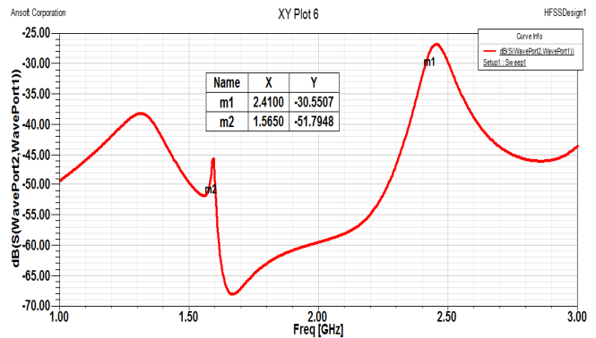
Figure 6: Isolation characteristics ( S21 ) of the two-element antenna array with and without CSS.
