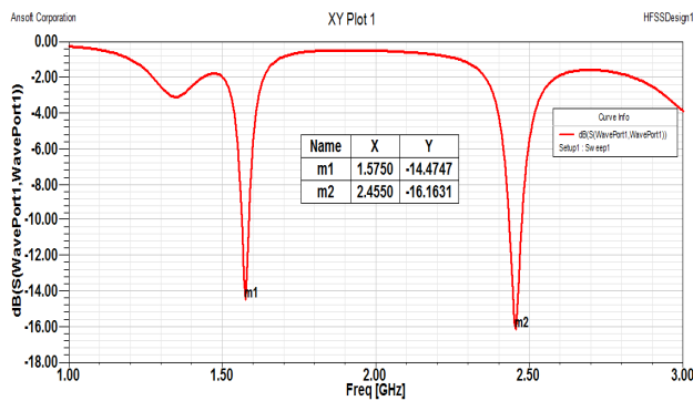
Figure 3. Return loss of proposed patch antenna
