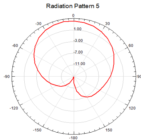
Figure 8. Radiation pattern
