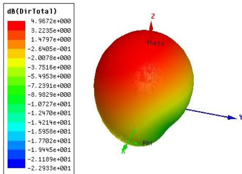
Figure 9. 3D Gain
