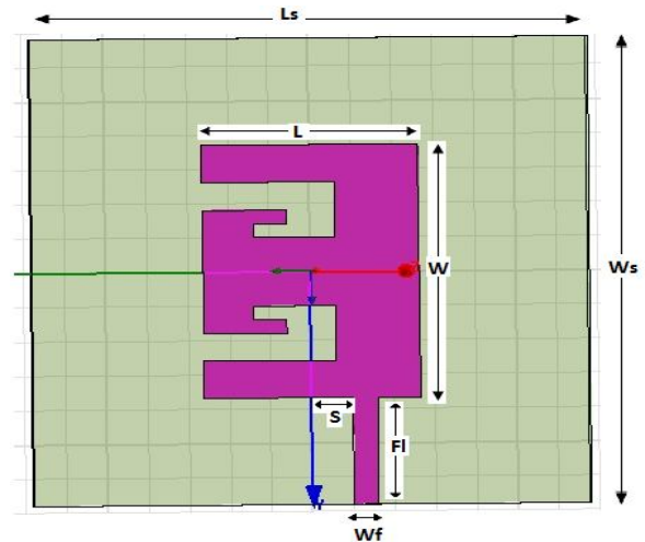
Figure 1. Geometry of the proposed Single double E shape patch antenna
