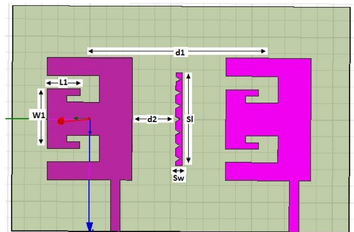
Figure 3. Proposed two-element antenna array with CSS decoupling unit.
