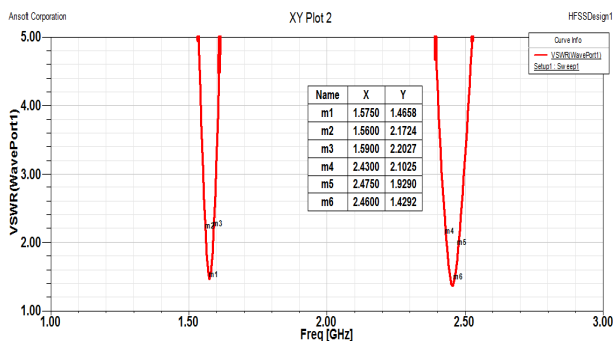
Figure 4 : VSWR of proposed patch antenna
