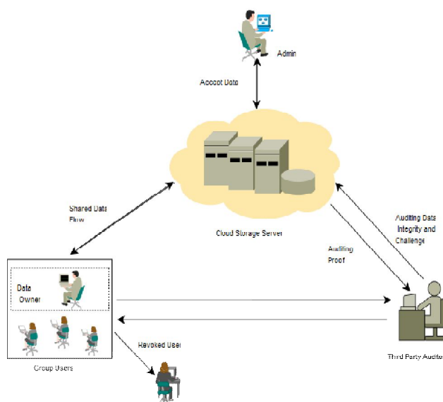
Figure 1: Architecture
