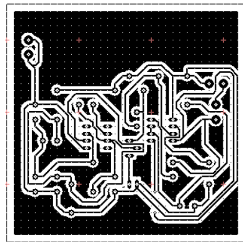
Fig.3 Artwork Layout of PCB
