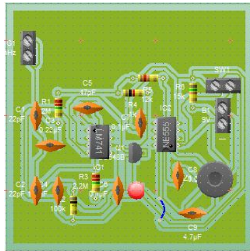
Fig.2 PCB Layout
