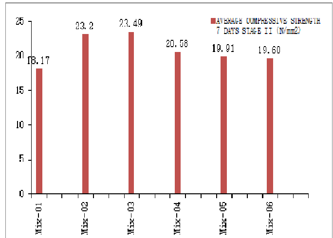
Figure 1. Compressive Strength in N/mm 2 at 7 days
