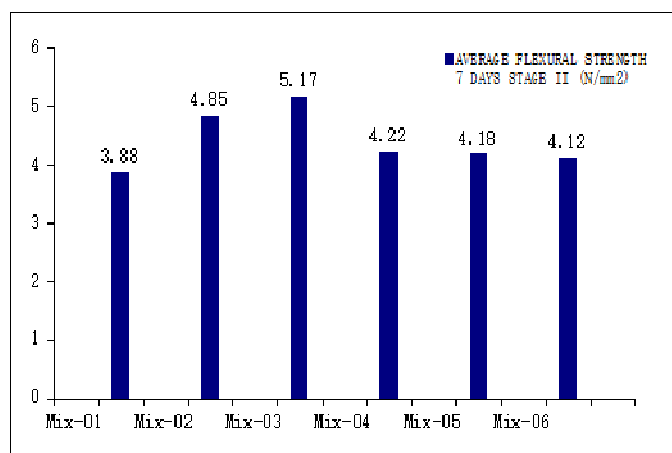
Figure 5. Flexural Strength in N/mm 2 at 7 days
