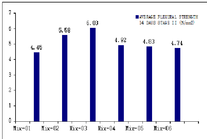
Figure 6. Flexural Strength in N/mm 2 at 14 days
