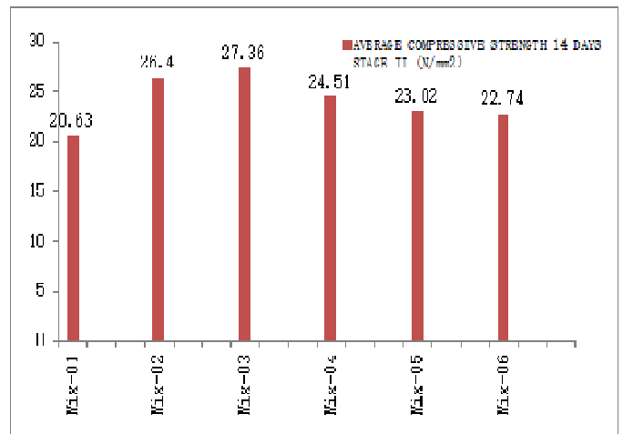
Figure 2. Compressive Strength in N/mm 2 at 14 days
