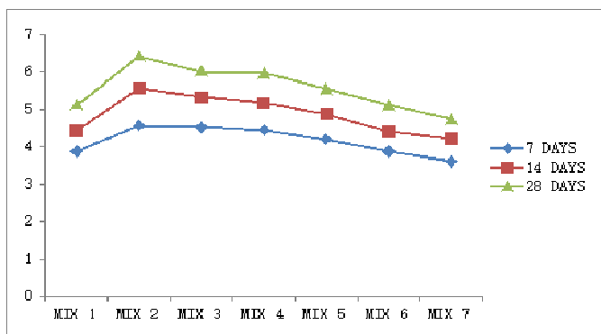
Graph 2: Flexural Strength in N/mm2 at various age (Days)
