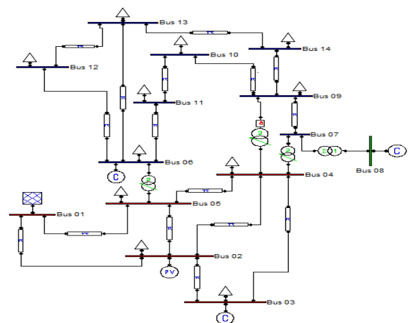
Fig.1: IEEE 14 Bus test system in PSAT
