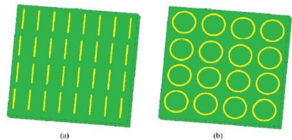
Figure 4. Typical single-layer two-dimensional frequency selective surfaces: (a, left) printed dipoles and (b, right) printed loops
