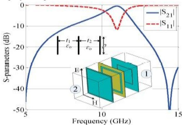
Figure 8. The S-parameter results of a cascaded combination of a bandpass and two band-stop frequency-selective surfaces (the variable names and geometry are consistent with those in Figures 4 and 5; w1 = 0.1\text{mm} , a1 = 9.3\text{mm} , w2 = 0.6\text{mm} , a2 = 8\text{mm} , w3 = 0.1\text{mm} , a3 = 5.6\text{mm} , p = 10\text{mm} , t1 = 4.5\text{mm} , t2 = 5\text{mm} ).
