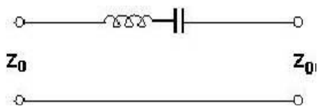
Figure 3. Simplest equivalent circuit representations of a band pass FSS in free space corresponding to a slot structure for one polarization and incidence angle.
