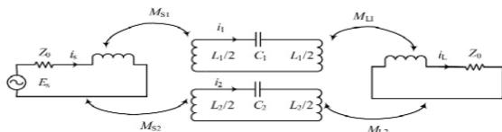
Figure 11. The equivalent circuit a dual-mode three-dimensional frequency-selective structure.
