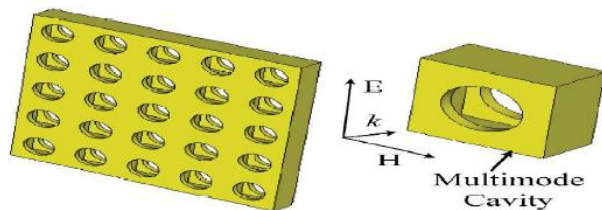
Figure 10. An illustration of a three-dimensional frequency selective surface consisting of a two-dimensional periodic array of multimode cavities.
