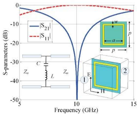
Figure 5. The S-parameter results and the equivalent circuit of a two-dimensional periodic array of printed loops ( w = 0.6\text{mm} , a = 7.3\text{ mm} , p = 10\text{ mm} ).
