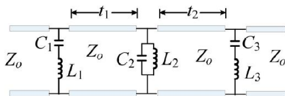
Figure 90. An equivalent circuit for the frequency-selective surface
