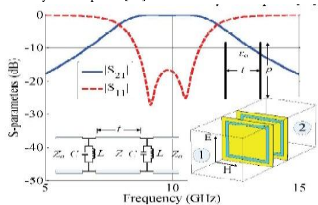
Figure 7. The S-parameter results and the equivalent circuit of a cascaded combination of two single-layer band pass frequency-selective surfaces of Figure 3 ( w = 0.6\text{mm} , a = 7.3\text{ mm} , p = 10\text{ mm} , t = 5\text{mm} ).
