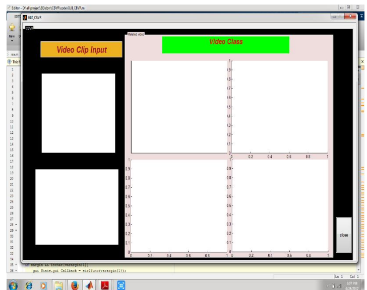
Figure 2. GUI
