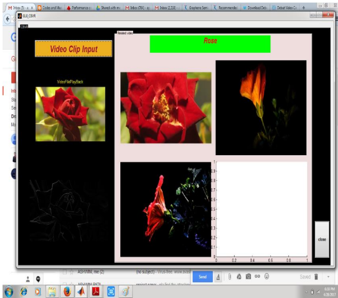
Figure 3. Retrieved video
