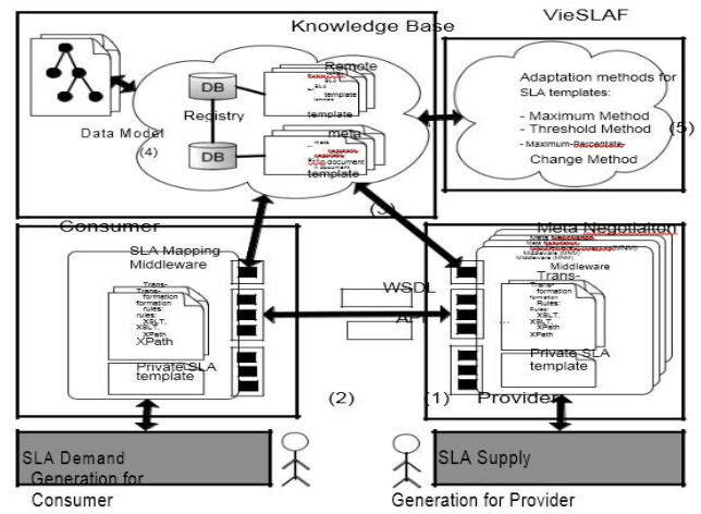
Figure 4. Adaptive SLA mapping architecture using VieSLAF.
