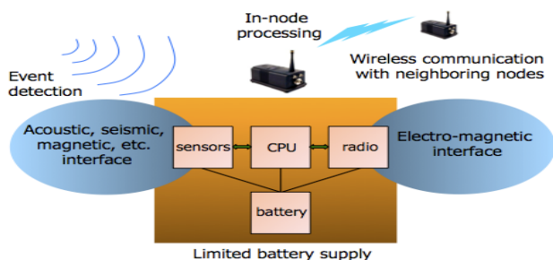
Figure 1. Components of WSN
