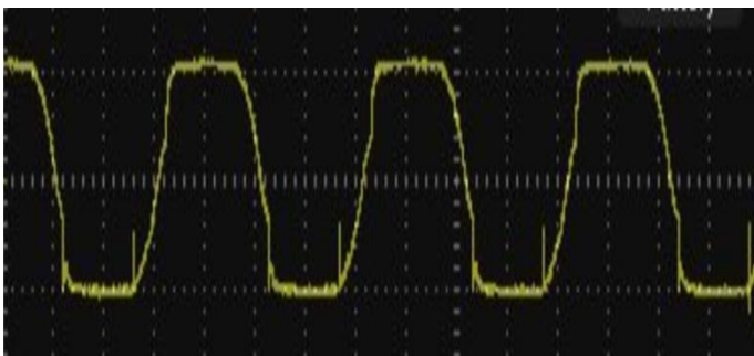
(4) With Resonant LC component
