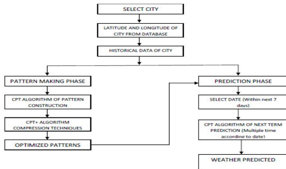
Figure 3: Prediction Architecture
