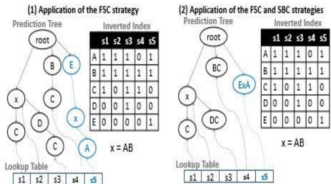
Figure 2: Compression Strategies
