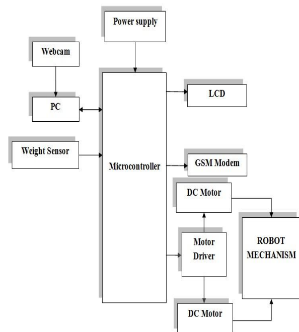
Fig1.System diagram
