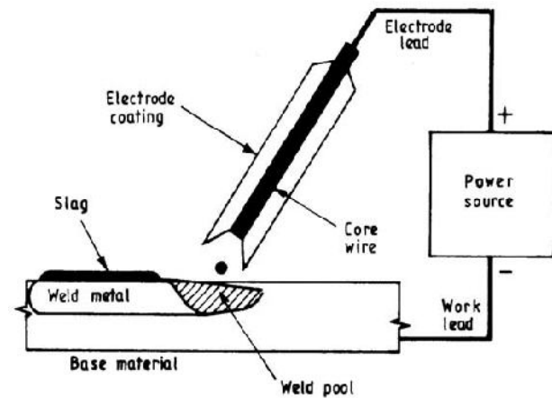
Figure 2: Schematic of shielded metal arc welding process
