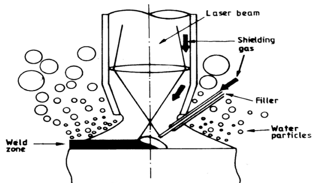
Figure 6: Schematic of laser welding with a filler rod.
