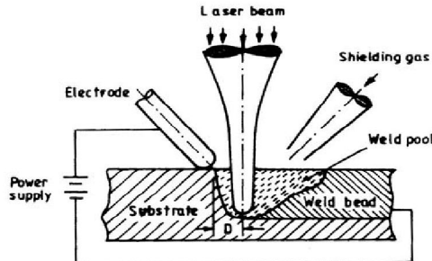
Figure 8: Schematic of experimental set-up for laser welding with an external current
