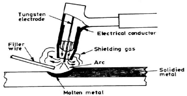
Figure 4: Schematic of a Gas Tungsten Arc Welding Technique
