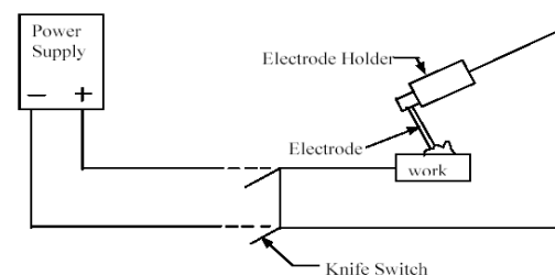
Figure 1: Hyperbaric welding
