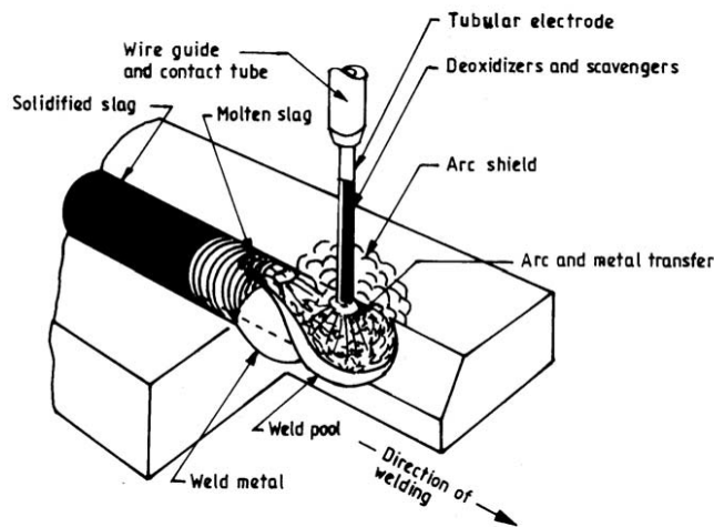
Figure 3: Schematic of Flux Cored Arc Welding
