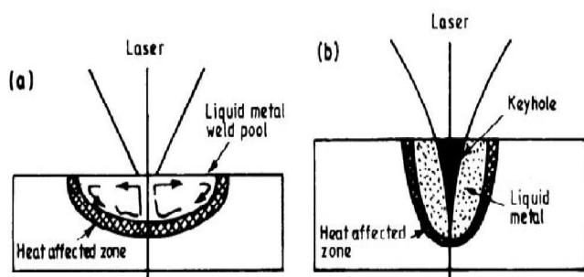
Figure 7: Schematic view of (a) Conduction melt pool, and (b) Deep penetration welding mode.
