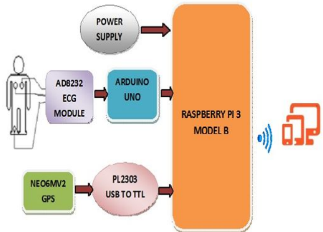
Figure 3. Block Diagram
