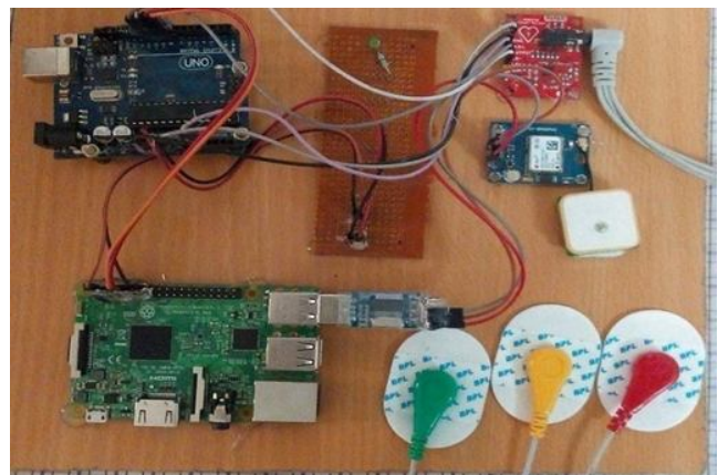
Figure 11. Experimental Setup
