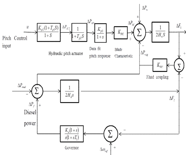
Fig. 1: Transfer function model block diagram of an isolated wind-diesel hybrid power system
