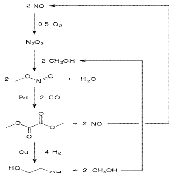
Fig 1 Methanol is recycled. Therefore only carbon monoxide, hydrogen, and oxygen are consumed
