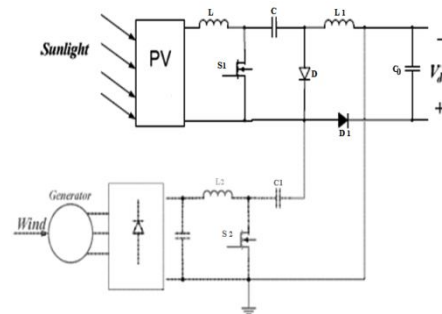
Fig.4 Only PV source is operational (Cuk)
