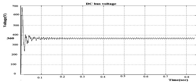
Fig.14 DC Link Voltage
