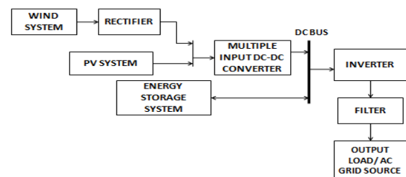
Fig. 1 Block diagram
