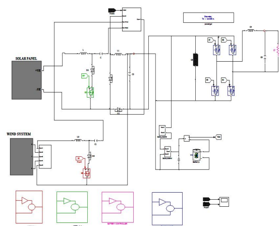
Fig.11 Hybrid system with Sepic-Cuk integrated converter
