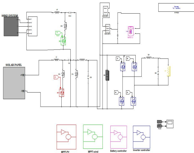
Fig. 8 Simulation circuit of Existing system
