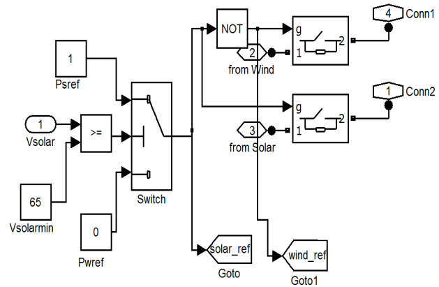
Fig. 7 Supervisory control circuit
