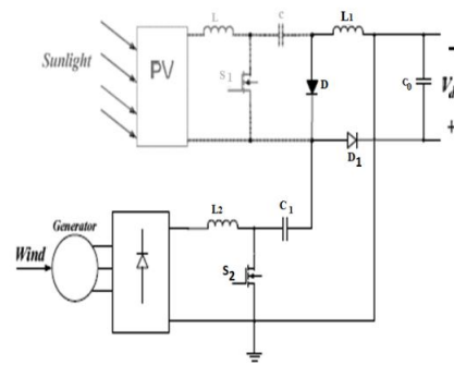
Fig.3 Only wind source is operational (SEPIC)
