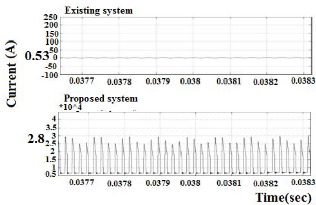
Fig. 16 Converter ripple current (PV)
