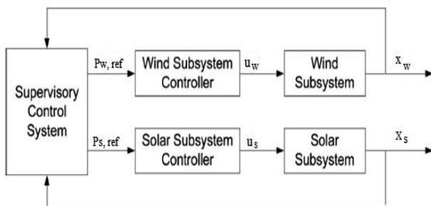
Fig. 6 Block diagram of Supervisory control system
