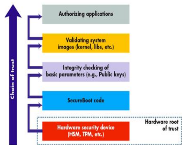
Figure 5. Generic secure boot architecture
