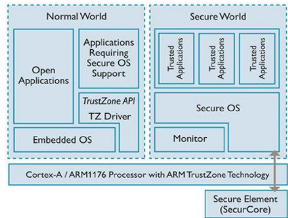
Figure 4. Trustzone software architecture
