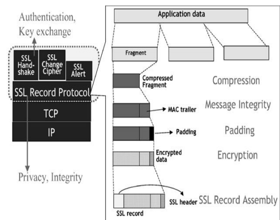
Figure 2. SSL protocol, with an expanded view of the SSL record protocol
