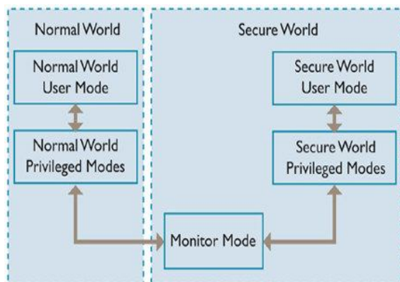
Figure 3. Trustzone hardware architecture
