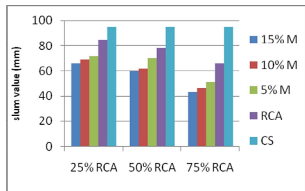
Graph 1: slum value experimental results
