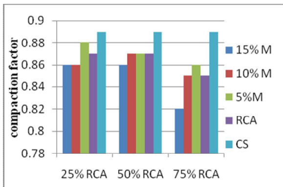
Graph 2: compaction factor experimental results
