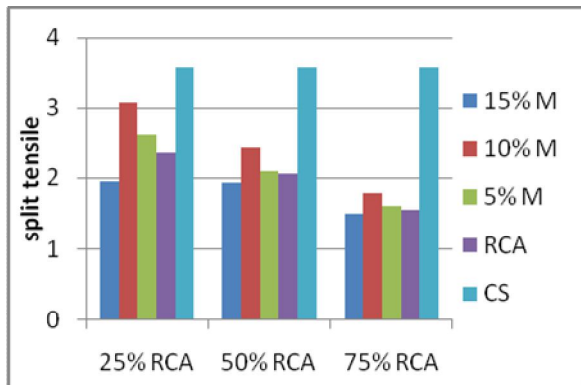
Graph 4: split tensile experimental results
