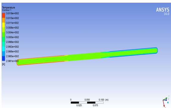
Fig 4.5 Temperature inside the tube.
