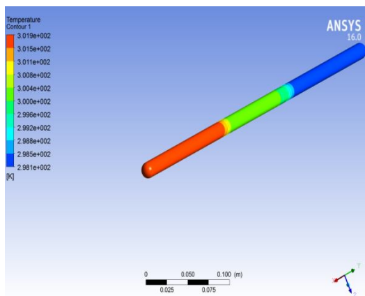
Fig 4.4 Temperature Contour.
