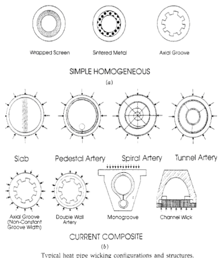
Fig 1.2 Capillary wick designs
