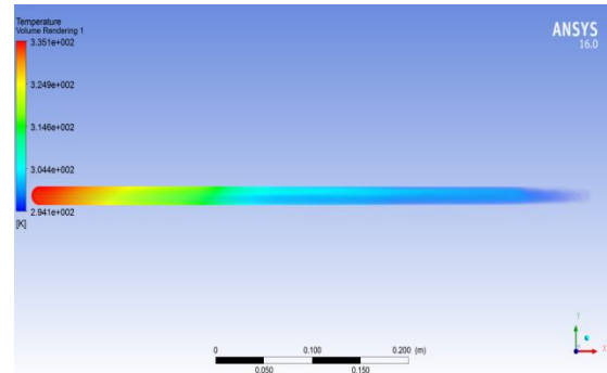
Fig 4.8 Temperature Distribution of 90 degree 102.9W.
