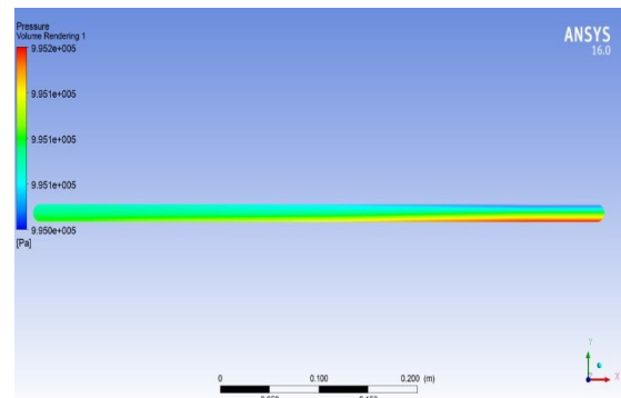
Fig 4.7 Pressure distribution of 90 Degrees 102.9W.
