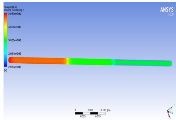
Fig 4.6 Temperature along the heat pipe.
