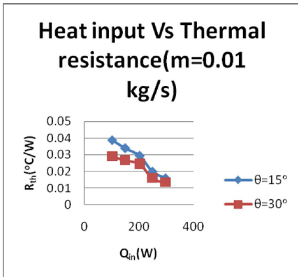
Graph 4.2 Heat input Vs Thermal resistance at m=0.01 kg/s
