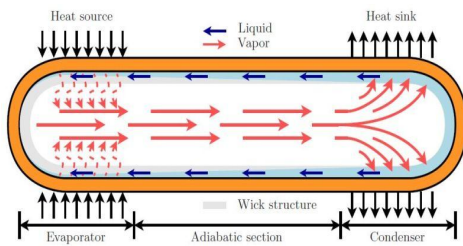
Fig 1.1 Principle of operation of heat pipe
