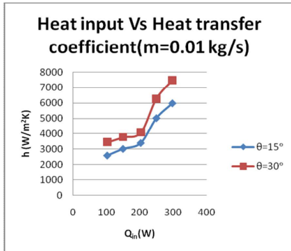
Graph 4.1 Heat input Vs Heat transfer coefficient at m=0.01 kg/s
