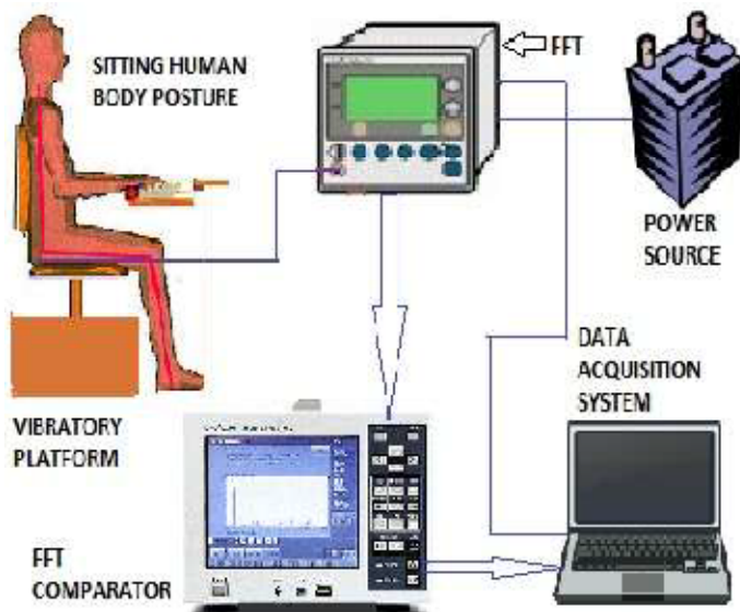
Fig.1. Experimental Setup()
