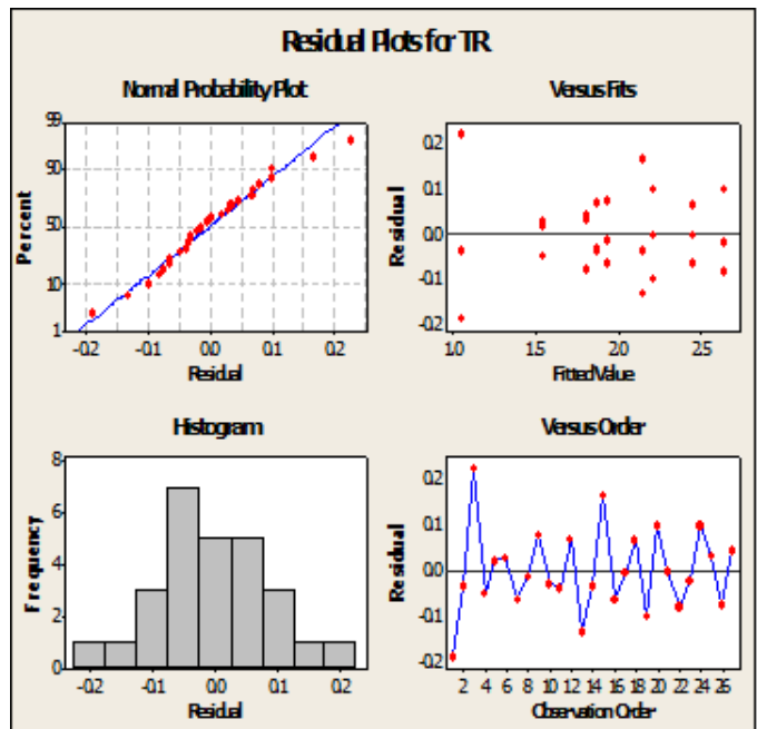
Fig. 3 Residual Plots for TR
