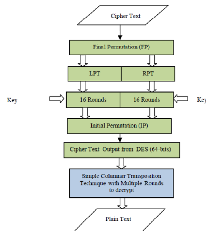
Fig.10. Decryption with Enhanced DES
