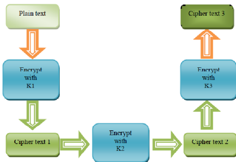
Fig.4. Encryption process Triple DES with three keys K1, K2 and K3
