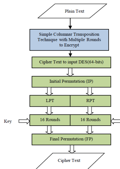
Fig.9. Encryption with Enhanced DES
