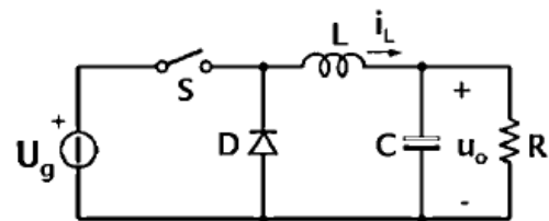
Fig.1 Buck Converter
