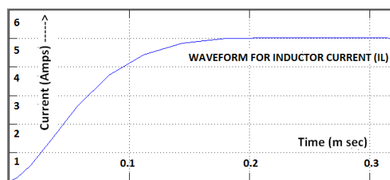
Figure. 17 Output Current waveform of Buck Converter using Sliding Mode Controller
