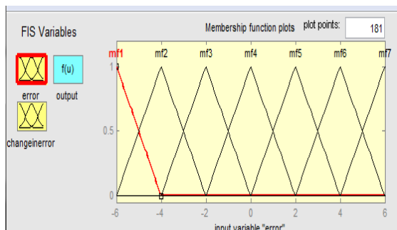
Figure 6. Membership functions for error normalized input
