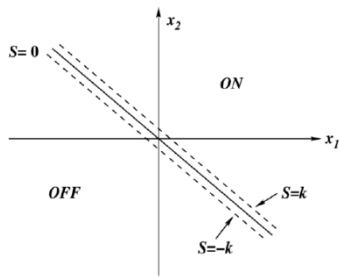
Figure 9. Sliding mode on x_1-x_2 phase plane
