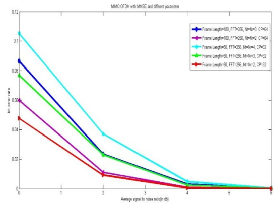
Figure.10: MIMO OFDM with MMSE and different parameters.
