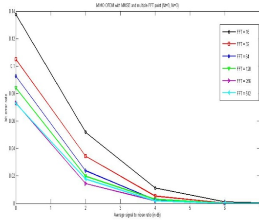
Figure.7: MIMO OFDM with MMSE and multi point FFT( N_t=3=N_r )
