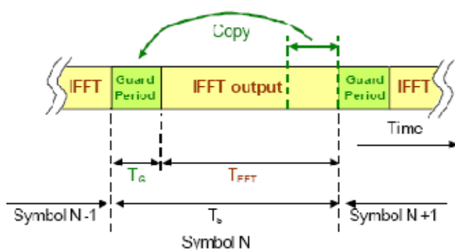
Fig. 2 Addition of a guard period to an OFDM signal
