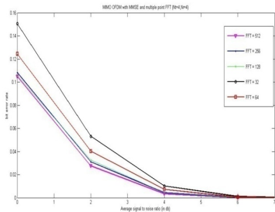
Figure.8: MIMO OFDM with MMSE and multi point FFT( N_t=4=N_r )
