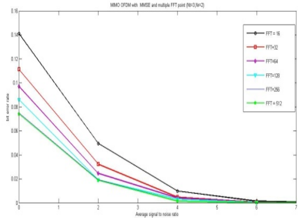
Figure.5: MIMO OFDM with MMSE and multiple FFT point( N_t=3, N_r=2 )
