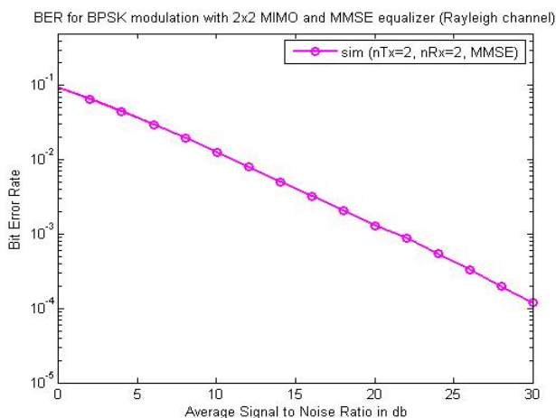
Figure 4: BER with MIMO and MMSE without OFDM
