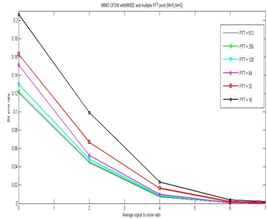
Figure.9: MIMO OFDM with MMSE and multi point FFT( N_t=5=N_r )
