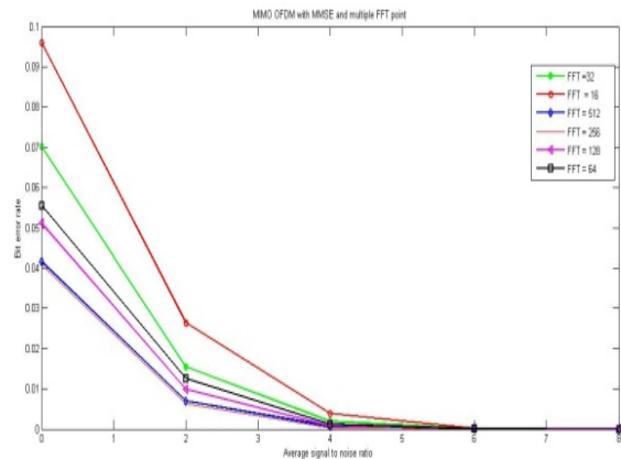
Figure.6: MIMO OFDM with MMSE and multi point FFT ( N_t=2=N_r )
