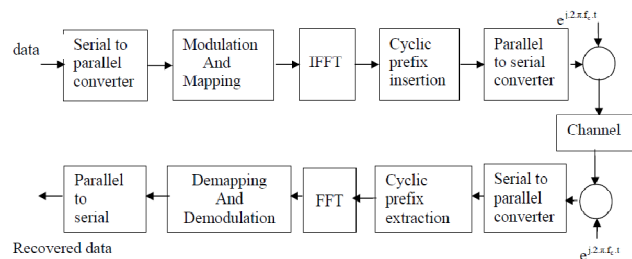
Fig 1. Block diagram of a basic OFDM transceiver.
