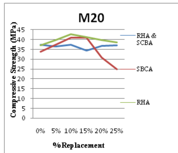
Figure 6 - Comparison Between Rha, Scba, Mixture Of Rha & Scba Of 28 Day Strength
