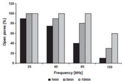
Fig 5. Open pores at different sonication frequencies and different exposure times [3]
