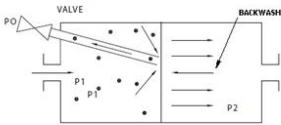
Fig 8. Schematic of forsta filter showing suction nozzle and valve [12].
