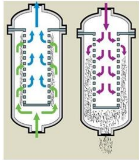
Fig 3. Schematic showing the regular and backwashing cycle of Eaton AFC, AFR & F-Series filters [2] .
