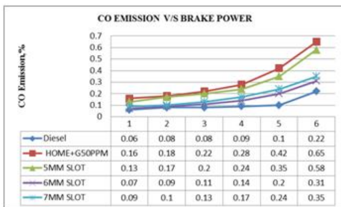
Figure 11: Variation of CO Emission with Brake power
