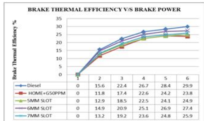
Figure 9: Variation of Brake Thermal Efficiency with Brake power
