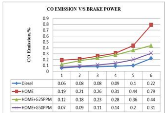
Figure 6: Variation of CO Emission with Brake power
