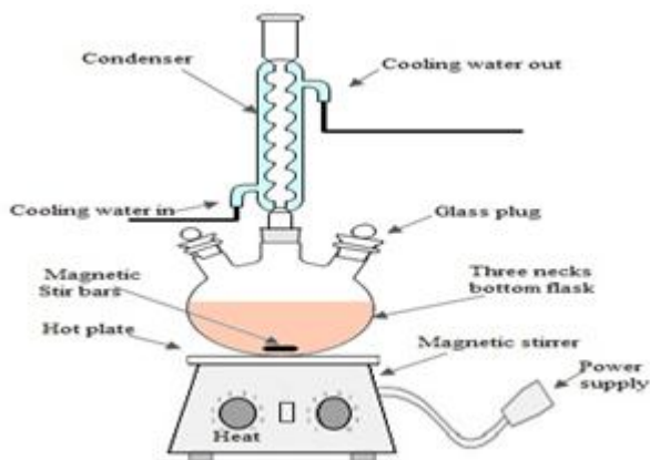
Figure 2: Transesterification setup
