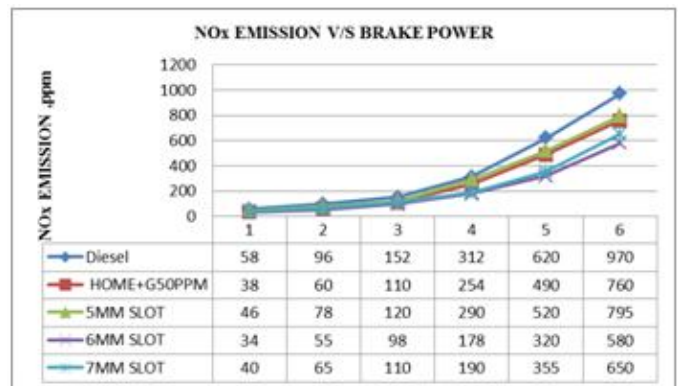
Figure 12: Variation of NOx Emission with Brake power
