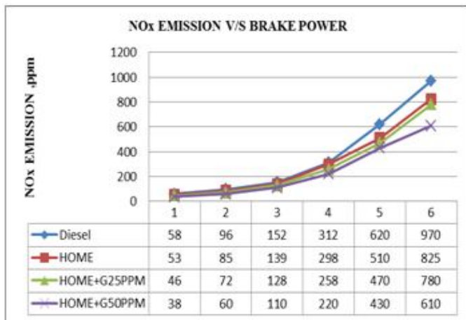
Figure 7: Variation of NOx Emission with Brake power
