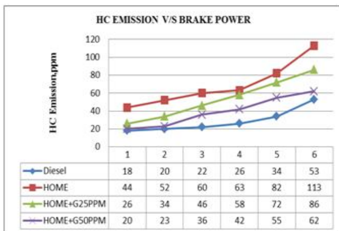
Figure 5: Variation of HC Emission with Brake power
