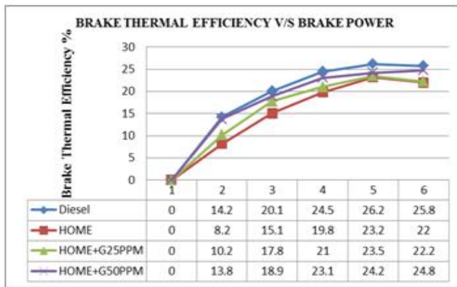
Figure 4: Variation of Brake Thermal Efficiency with Brake power
