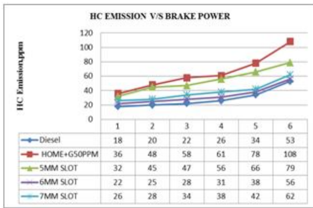
Figure 10: Variation of HC Emission with Brake power
