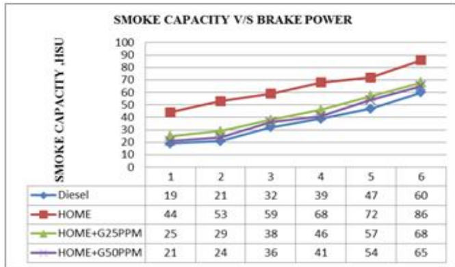
Figure 8: Variation of smoke capacity with Brake power
