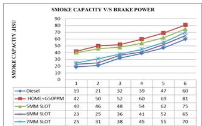
Figure 13: Variation of smoke capacity with Brake power
