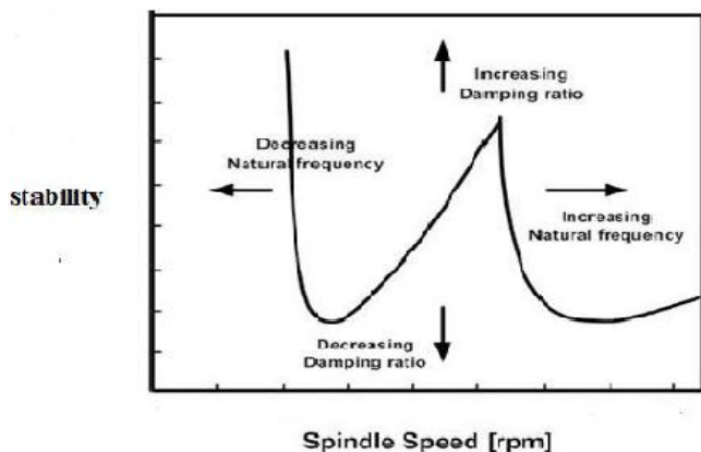
FIG 7: Stability lobe behavior according to natural frequency and damping ratio [11]
