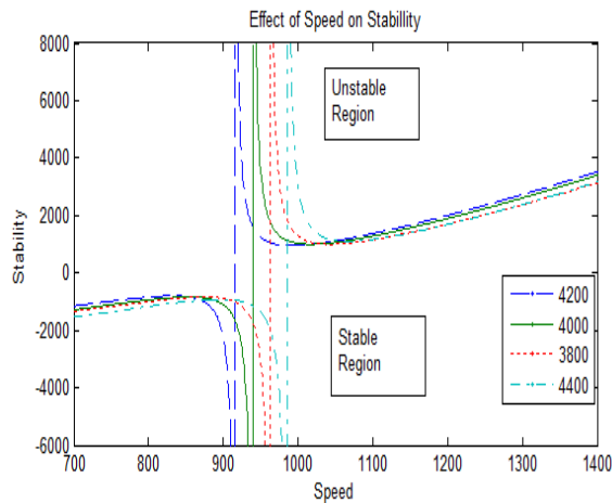
FIG 6: Effect of speed on stability for different stiffness
