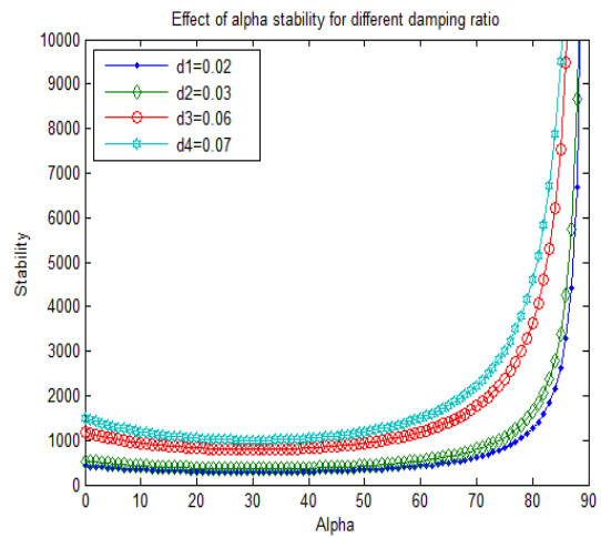
FIG 4 : Effect of \alpha on stability for different damping ratio
