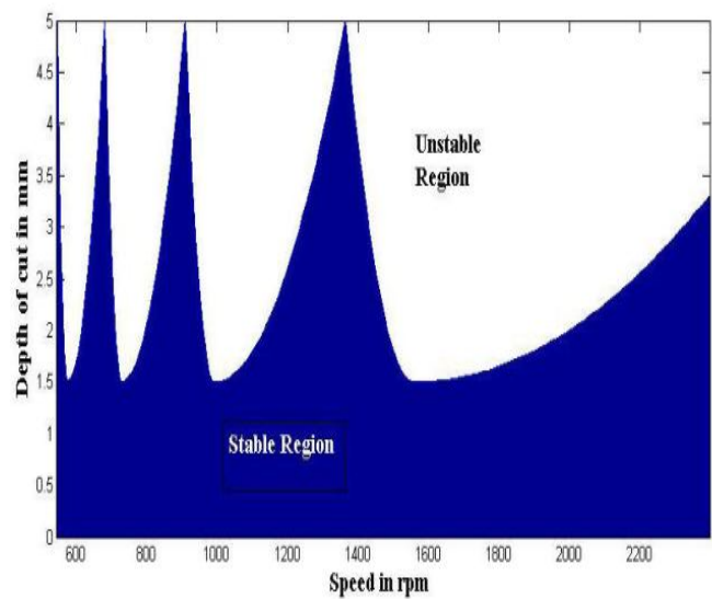
FIG 8 : Stability Lobe Diagram for hard turning
