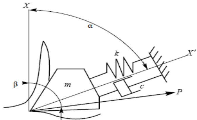
FIG 1: Single Degree of Freedom turning operation [15]
