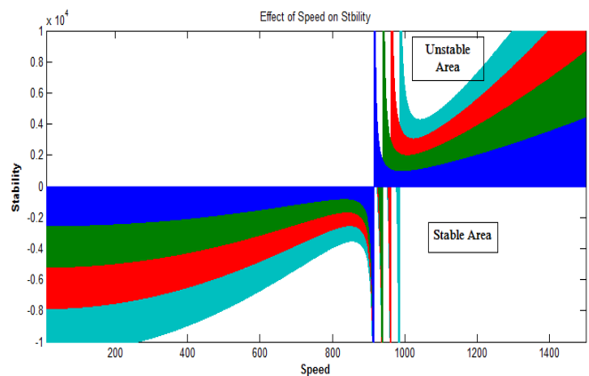
FIG 5: Effect of speed on system stability for different damping ratio
