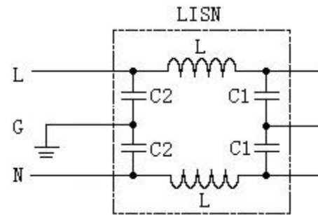
FIGURE 1.1 SCHEMATIC DIAGRAM OF LISN
