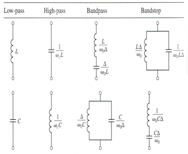
FIGURE 1.2 TRANSFORMATIONS
