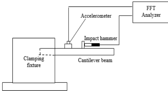
Fig 1. Experimental set up Block diagram
