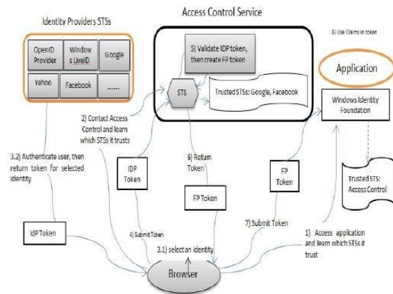
Figure 6. The access control service makes it easier for an application to accept identities from multiple cloud identity providers [6]
