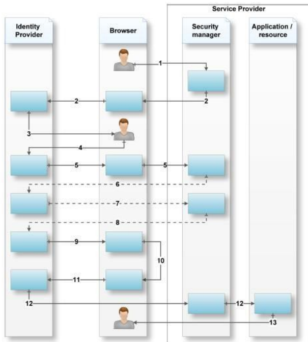
Figure 2. Adaptation of current federated identity management tools [2]
