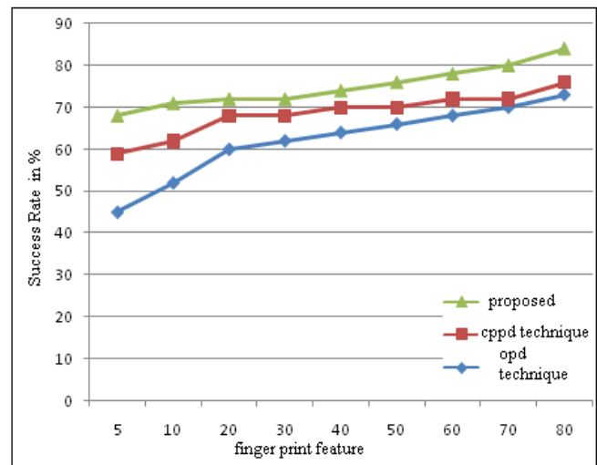
Fig. 3. Reconstruction techniques comparison.
